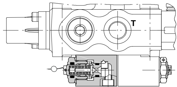
H: valve set and locked
